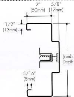
Double Rabbet
