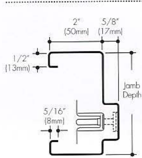
Single Rabbet
